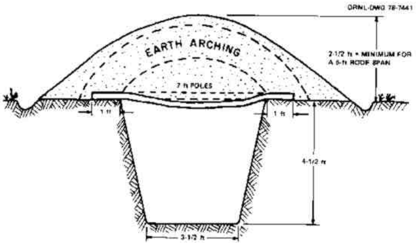
Fig. 5.7. Earth arching over a yielding roof enables a shelter to withstand much greater pressures. ORNL.DWG 78.7441
