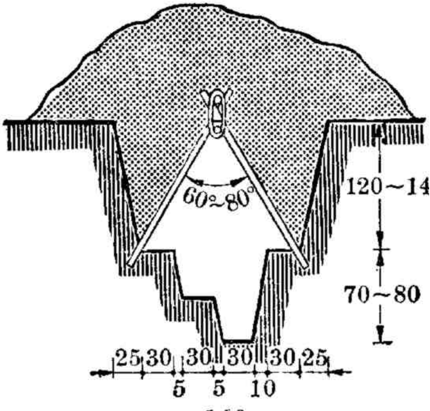
Fig. D.9. Chinese "Man" Shelter tested at 20 psi, and undamaged because the thin poles yielded and were protected by earth arching. This drawing was taken from a Chinese civil defense manual. The dimensions are in centimeters.
