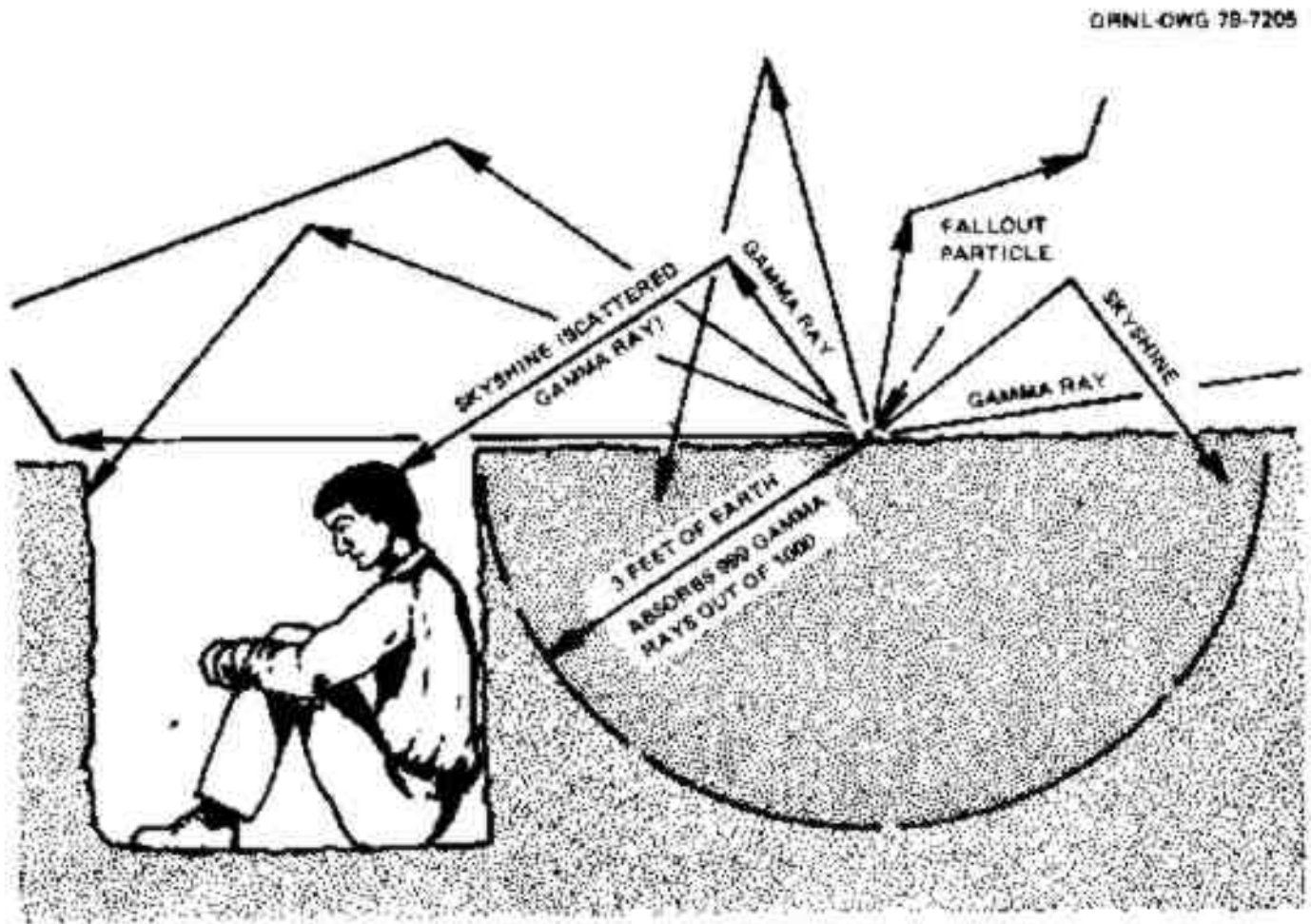
Fig. 5.3. Simplified illustration of barrier shielding and skyshine (scattered gamma radiation). An open trench provides poor protection. ORNL.DWG 78-7205
