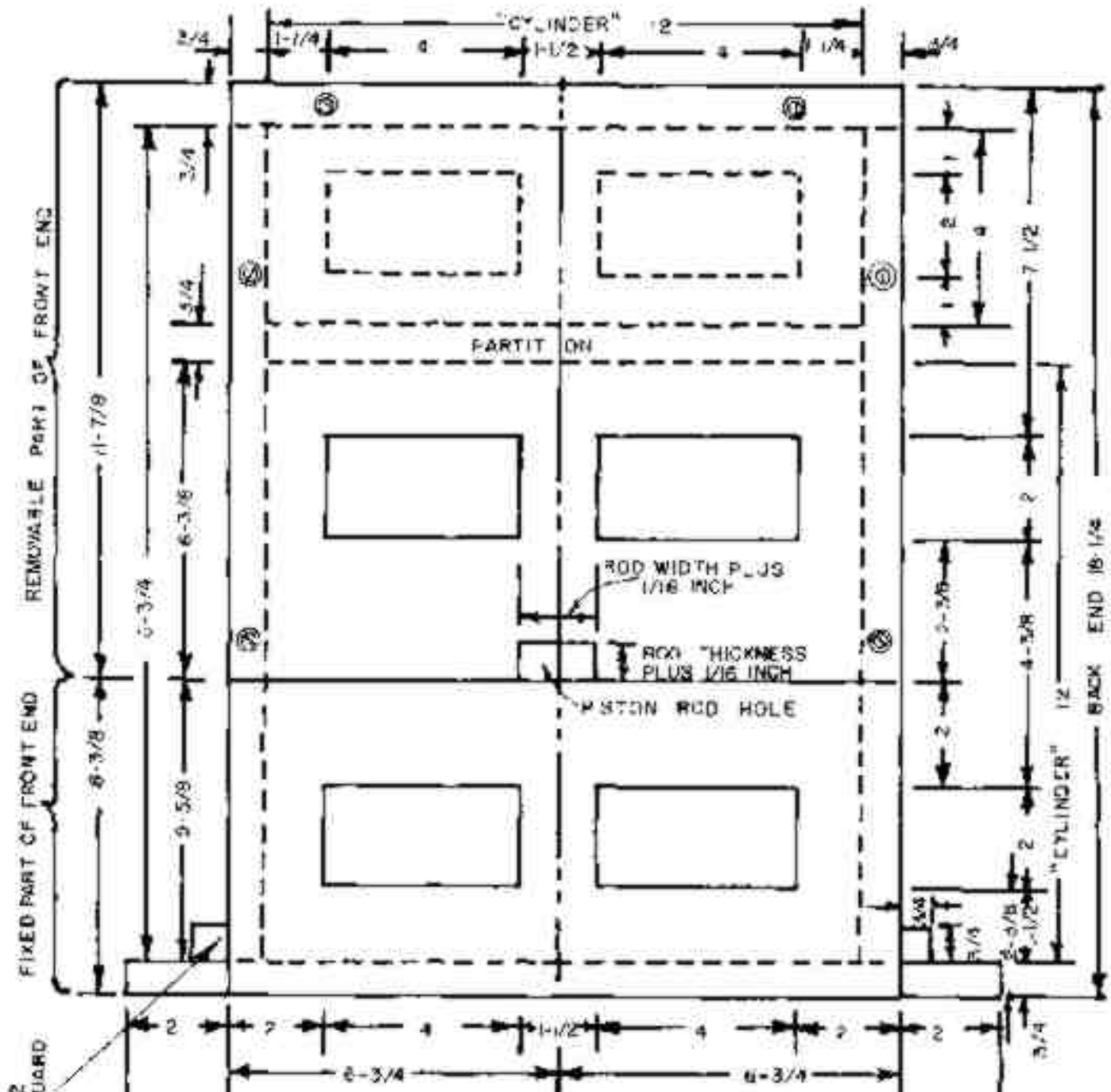
Fig. 8. Back End. Only the plywood is shown.
