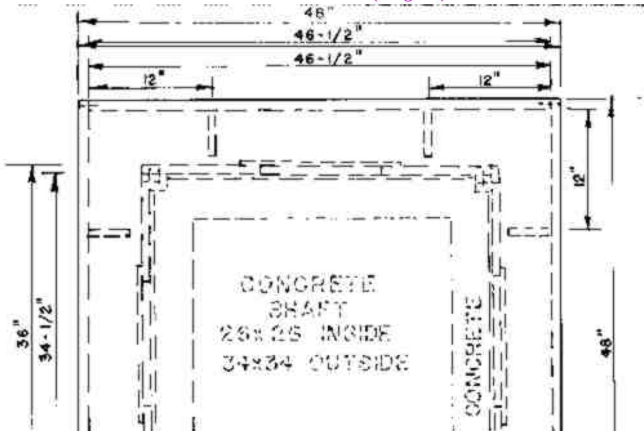
Fig. F.2. Plan and Side View of Multi- Purpose Emergency Exit Housing, on a Square Emergency Exit with 34 x 34-Inch Cross- Sectional Outside Dimensions. (Diagram)
