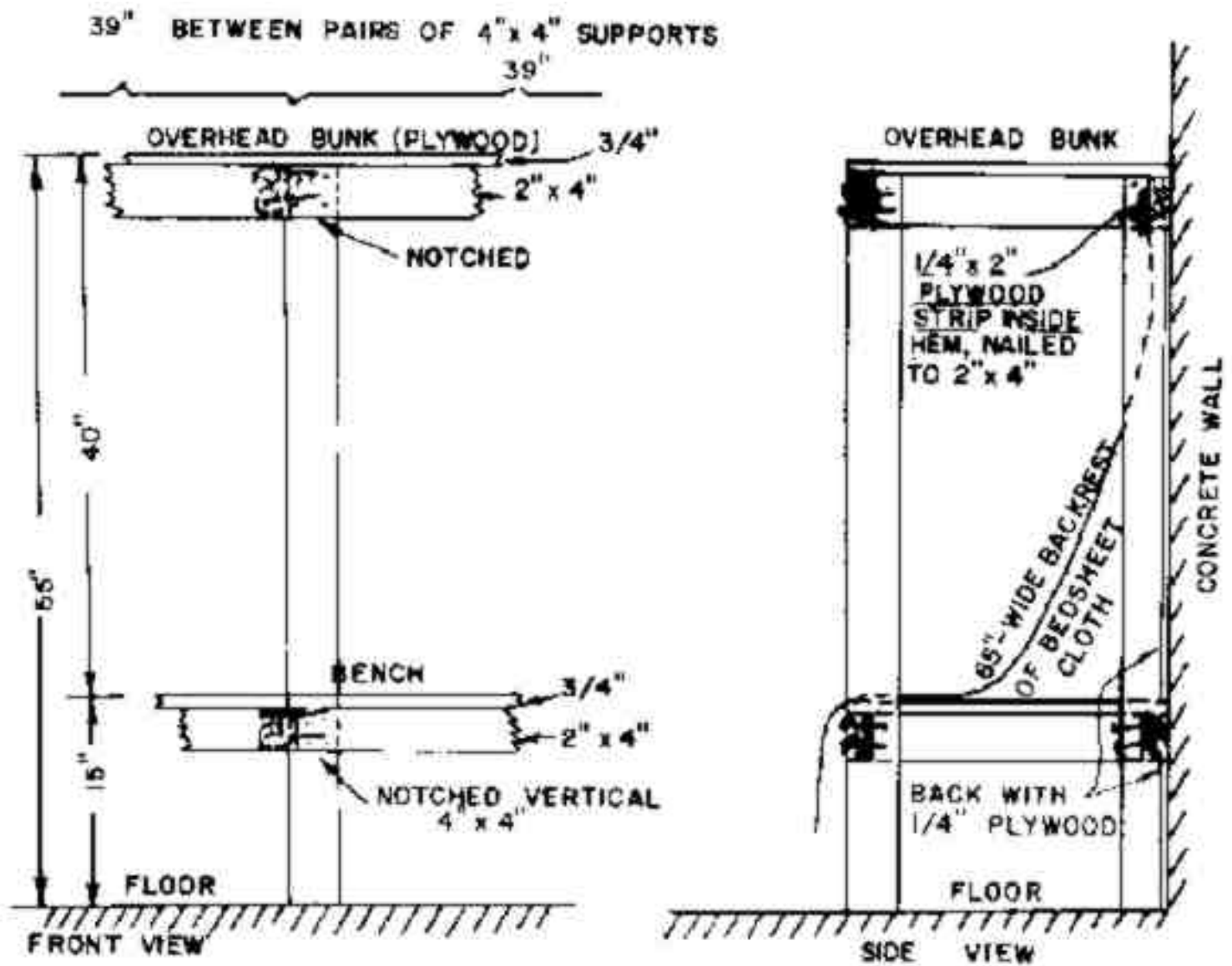
Fig. 17.5. Backrests of Bedsheet Cloth and 2-Inch-Thick Pads Make Sitting and Sleeping Comfortable.
