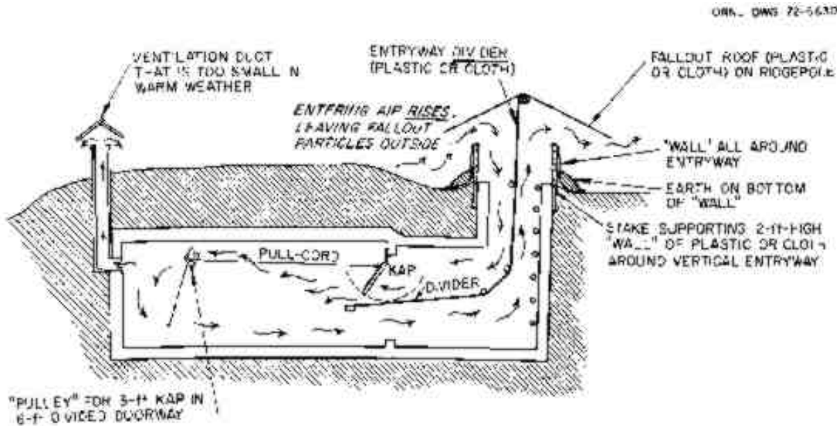
Fig. 15. Ventilating a shelter when the air-exhaust opening is too small. ORNL DWG 72-6630
