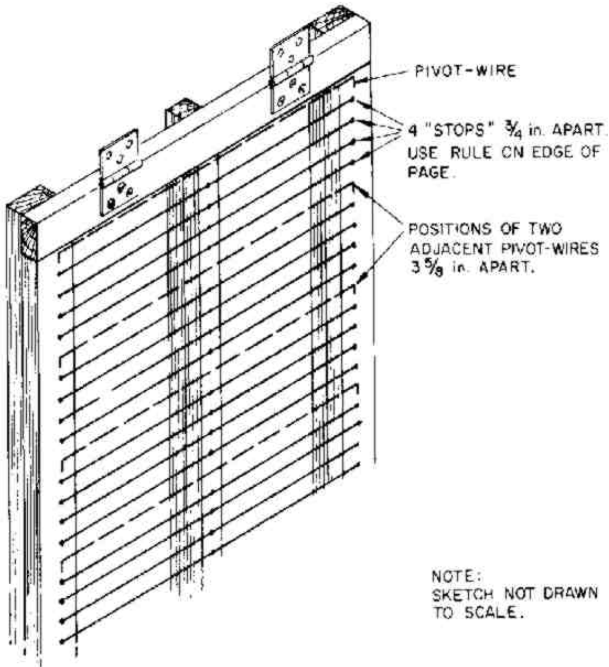
Fig. 11. Positions of pivot-wires and flap-stops.
