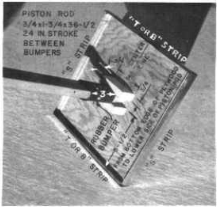
Fig. 14. Plywood Piston with Sheetmetal Sealing Strips Attached.
