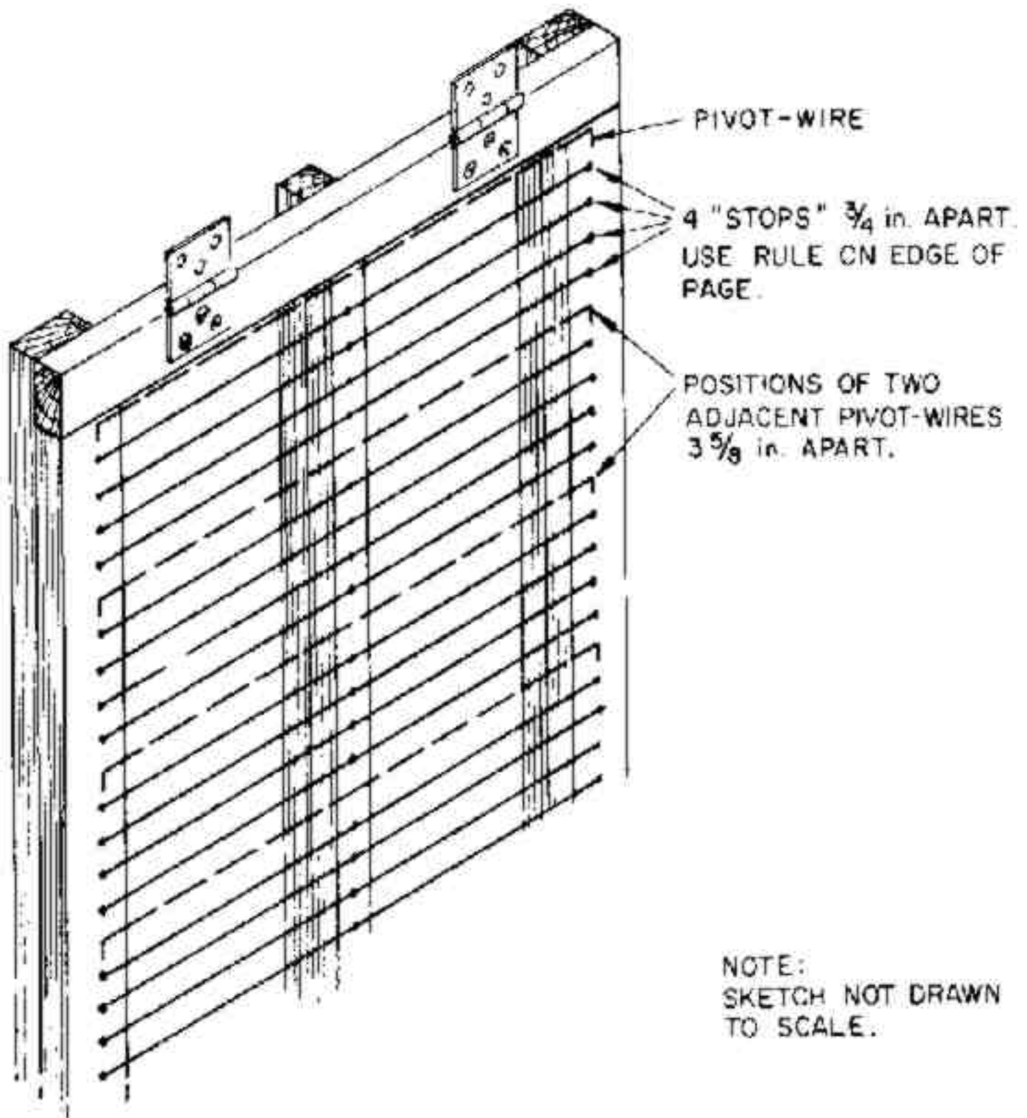
Fig. 11. Positions of pivot-wires and flap-stops.
