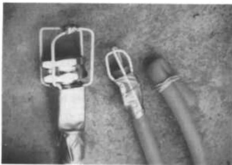
Fig. 8.8. Two wire "protectors," each made of two pieces of coathanger wire taped to a 1/2 inch flexible hose and a rubber tube. Shown on the right is a tube closed with a rubber band to stop a siphoned flow of water. (Illustration)
