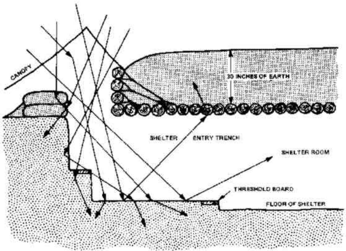
Fig. 5.6. Earth mounded over a 3 foot-wide Pe-Covered Trench Shelter. The canvas canopy would protect the vertical entry against both fallout and rain. (A smaller canopy over the air duct-emergency exit at the other end is obscured by the mounded earth.)
