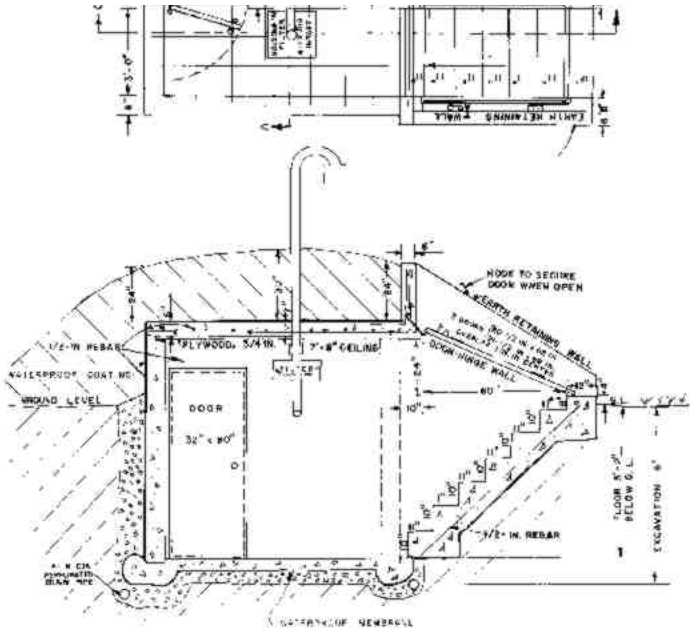
Fig. 17.1. Permanent Family Fallout Shelter for Dual Use.
