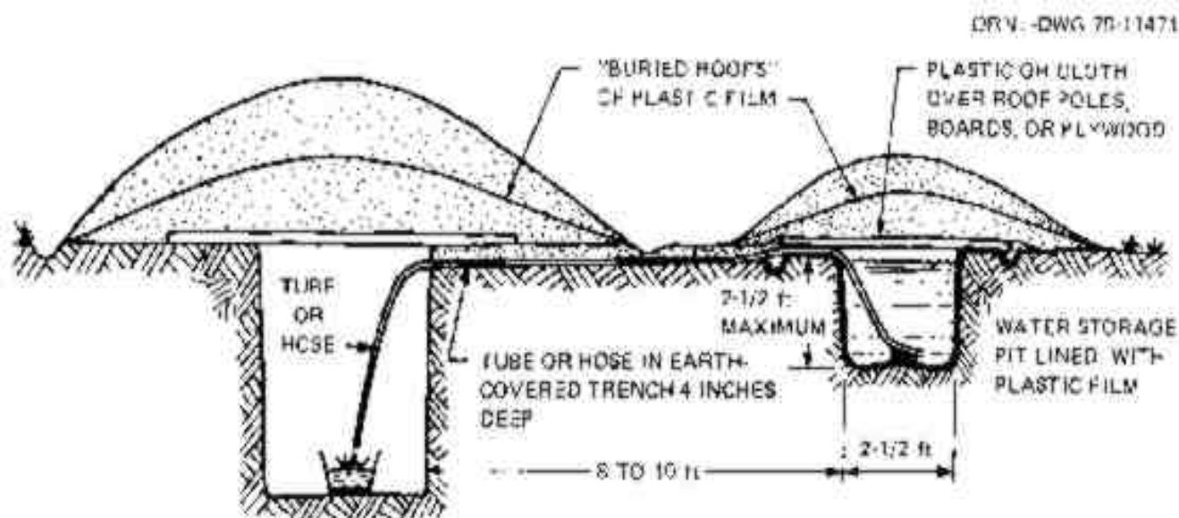
Fig. 8.7. Water siphoned into a belowground shelter. ORNL-DWG 78-11471 (Illustration)
