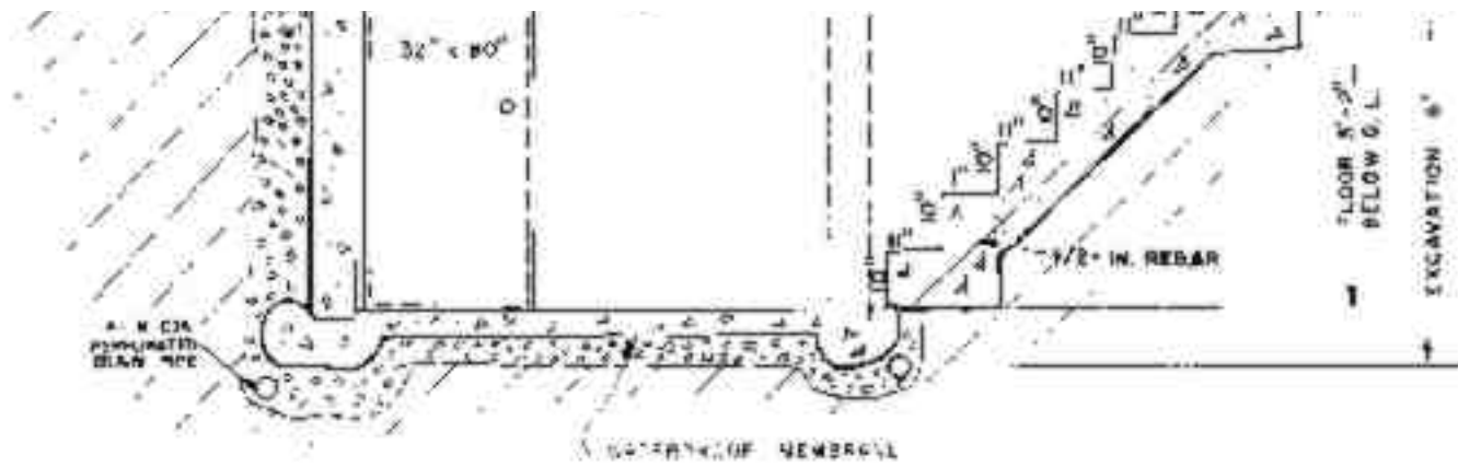
Fig. 17.1. Permanent Family Fallout Shelter for Dual Use.
