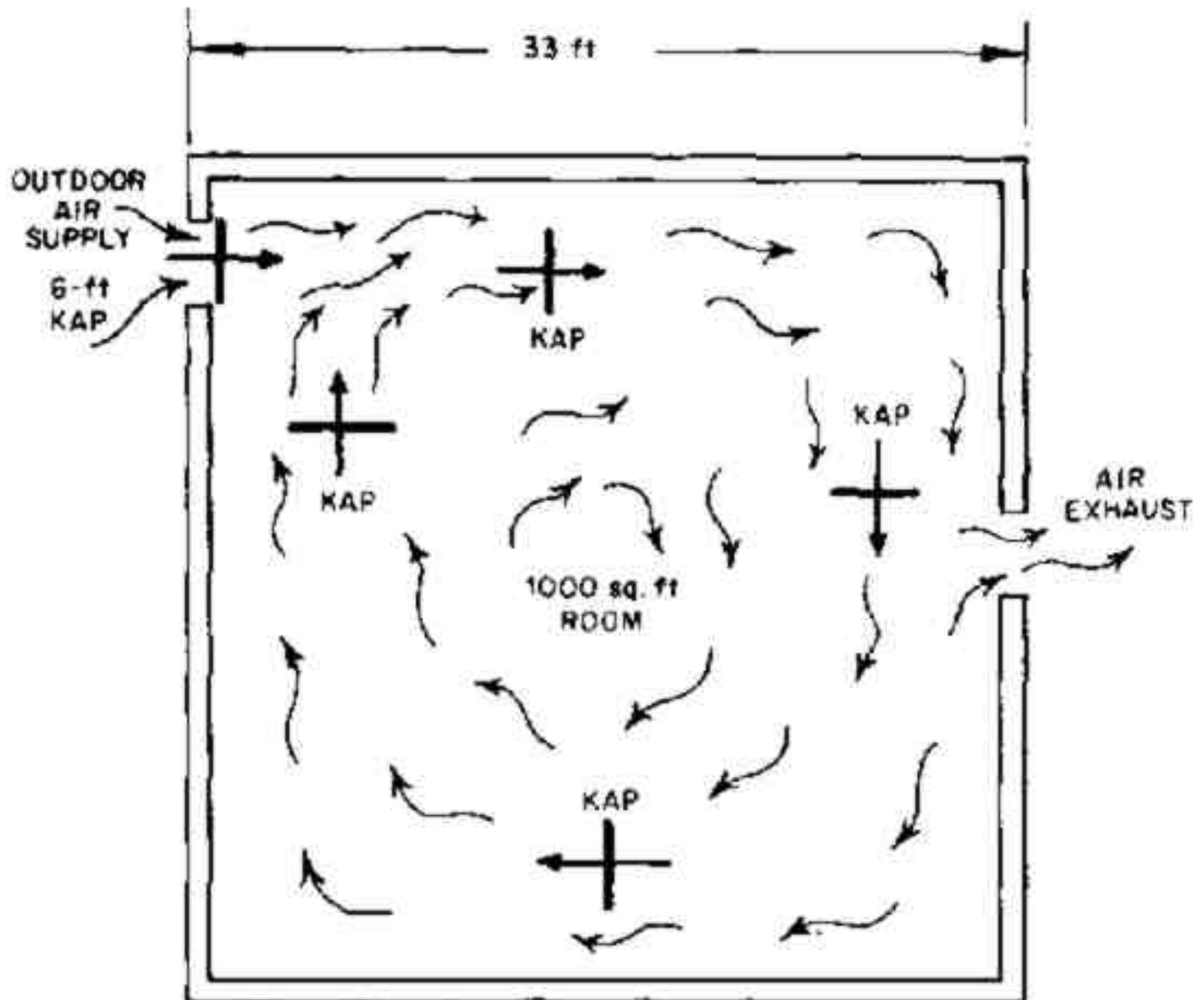
Fig. 16. The use of air-distribution KAPs.
