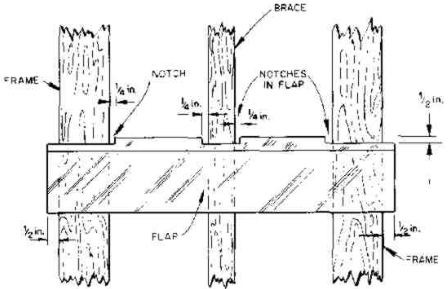
Fig. 6. Sizes of notches in flaps.
