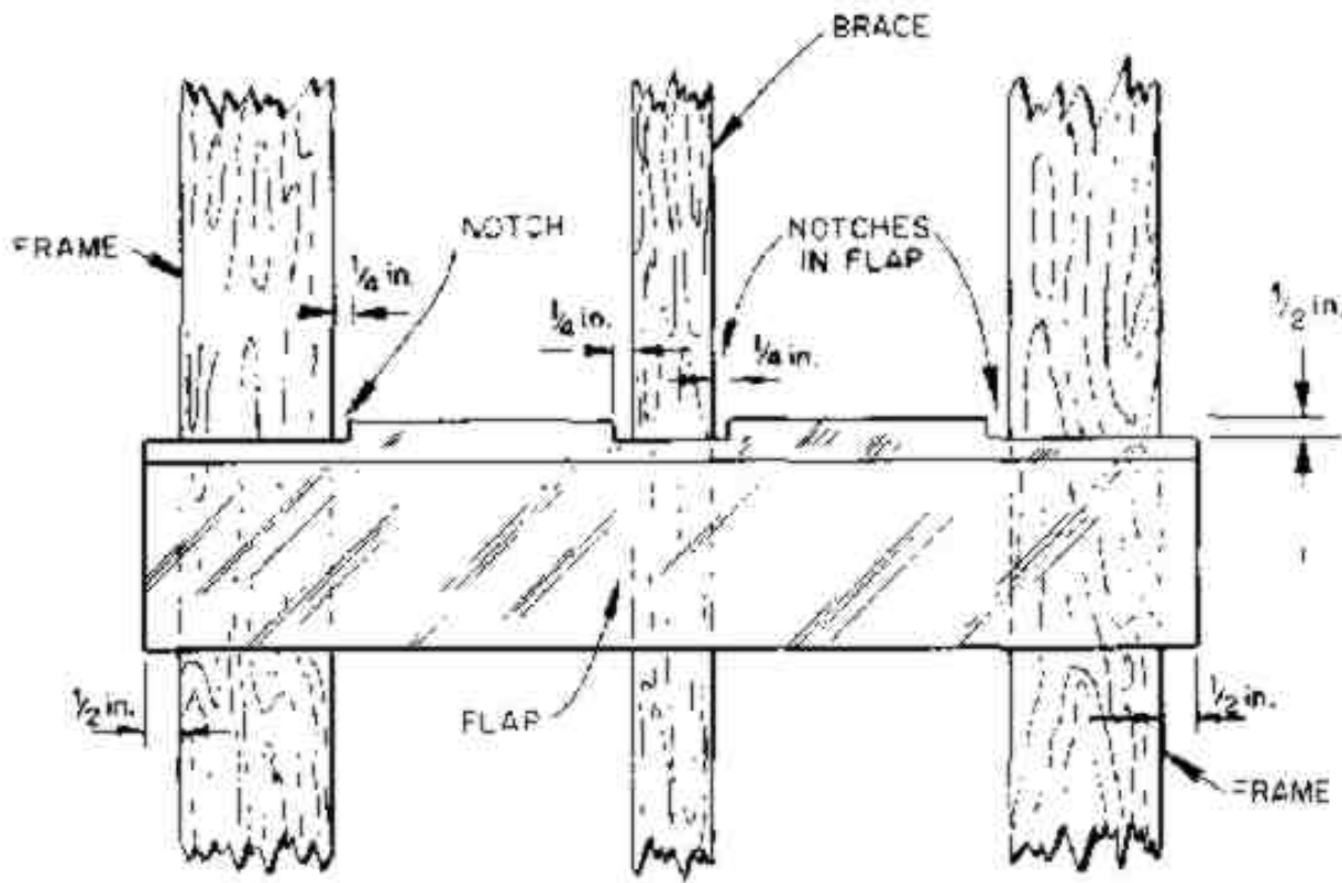
Fig. 6. Sizes of notches in flaps.
