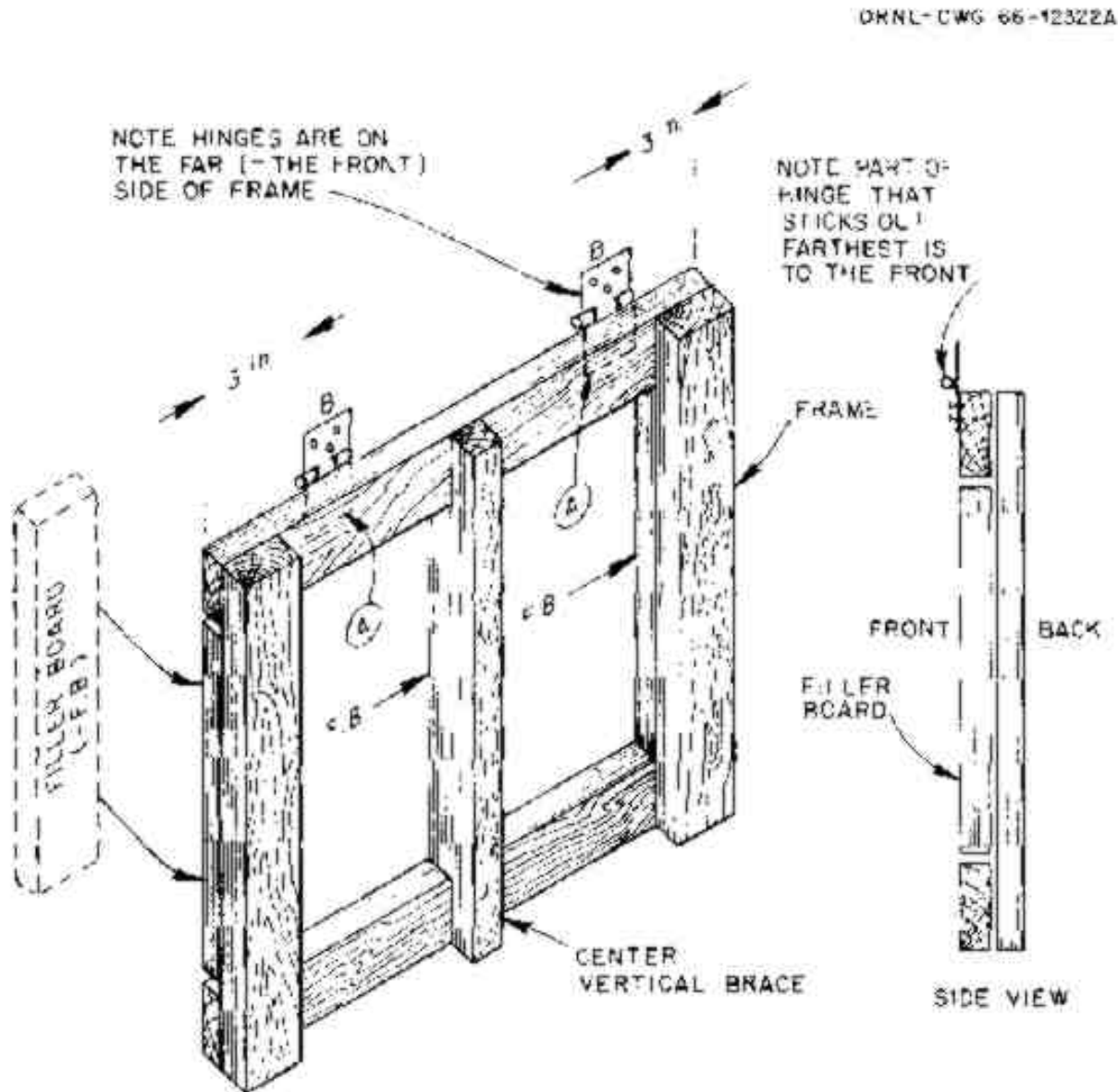
Fig. 4. Completing the frame. ORNL- DWG 66-12322A
