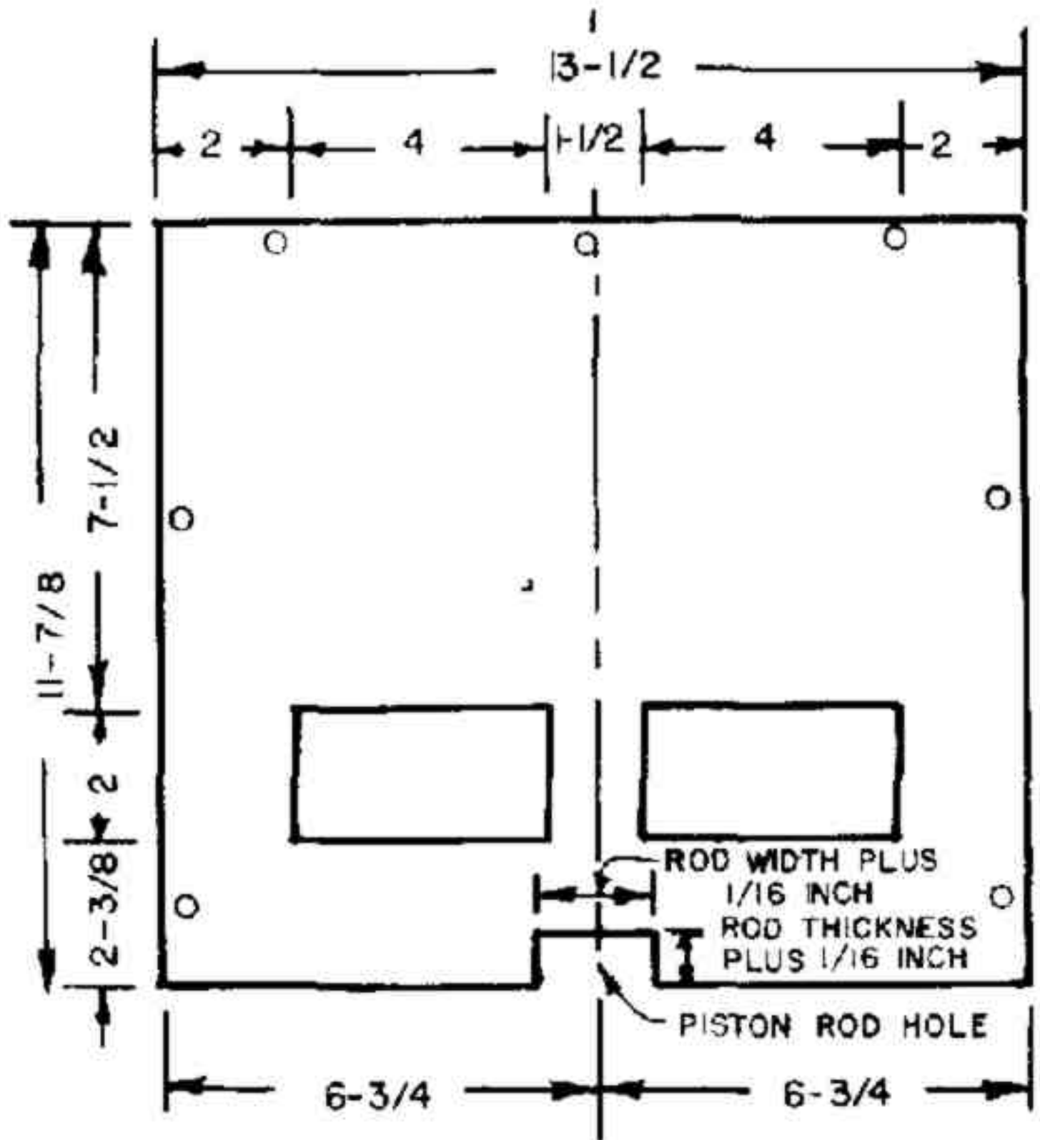
Fig. 10. Fixed Part of Front End, Unfinished. Only the plywood is shown.
